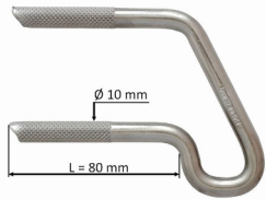
Art. 522 Fork Ø 10 mm x 80 mm
